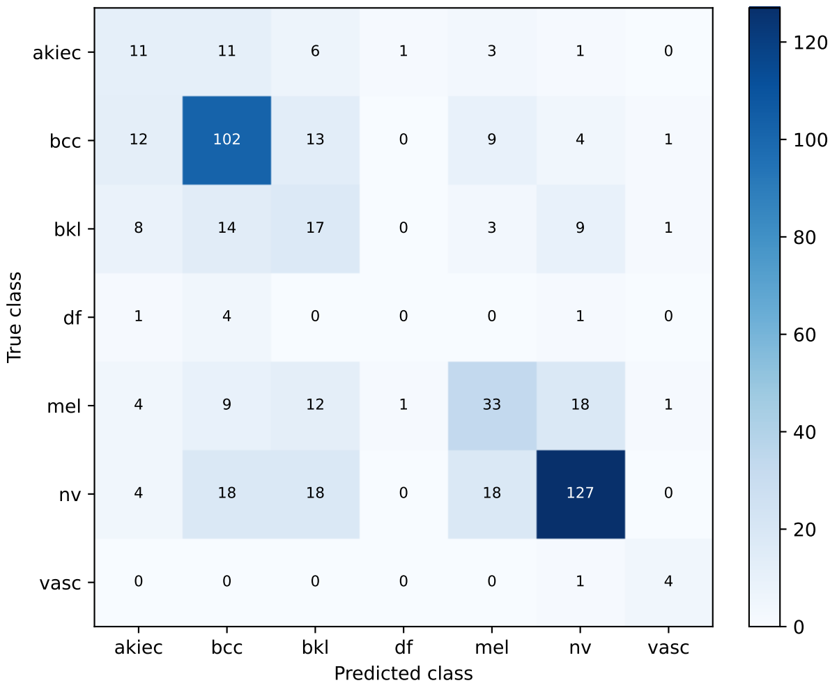
S66 ham_plus_external | external preflight domain check Confusion matrix
