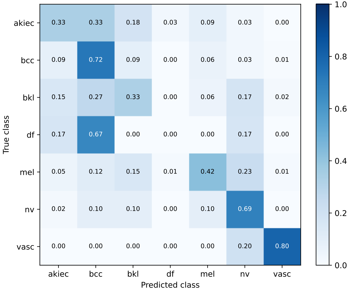
S66 ham_plus_external | external preflight domain check Row-normalized confusion matrix
