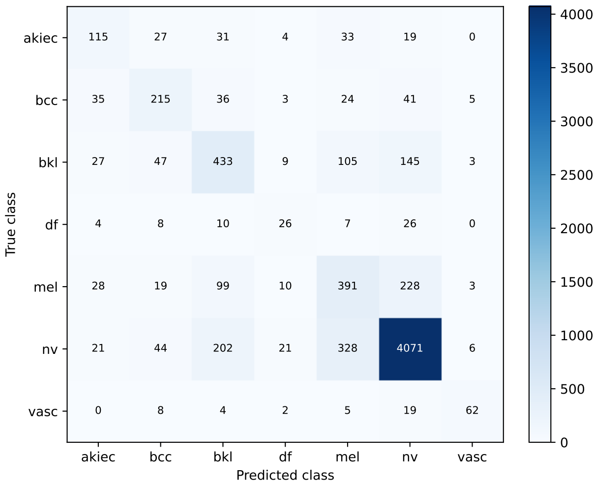
S67 ham_only | train-only lesion-group OOF Confusion matrix
