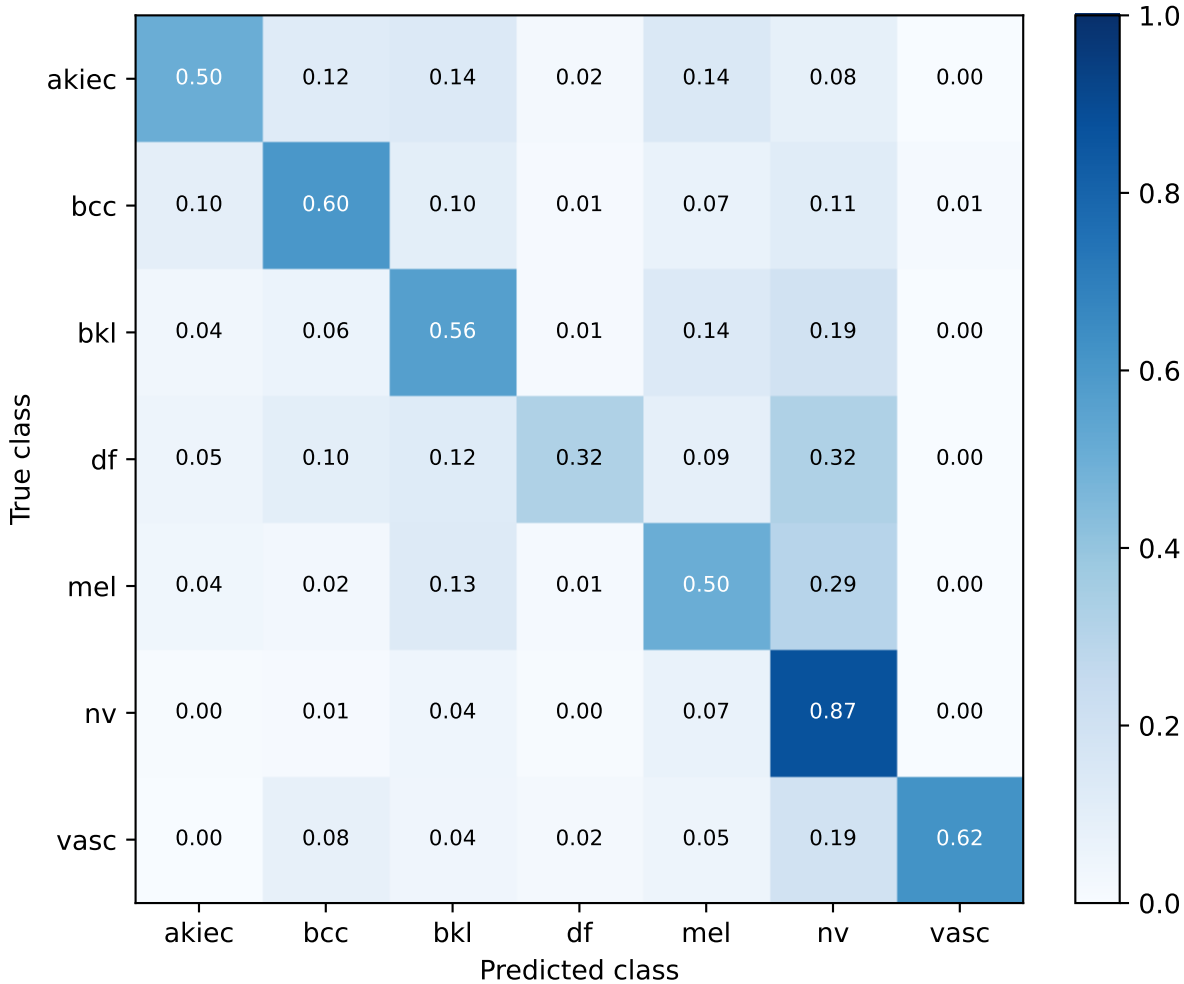
S67 ham_only | train-only lesion-group OOF Row-normalized confusion matrix
