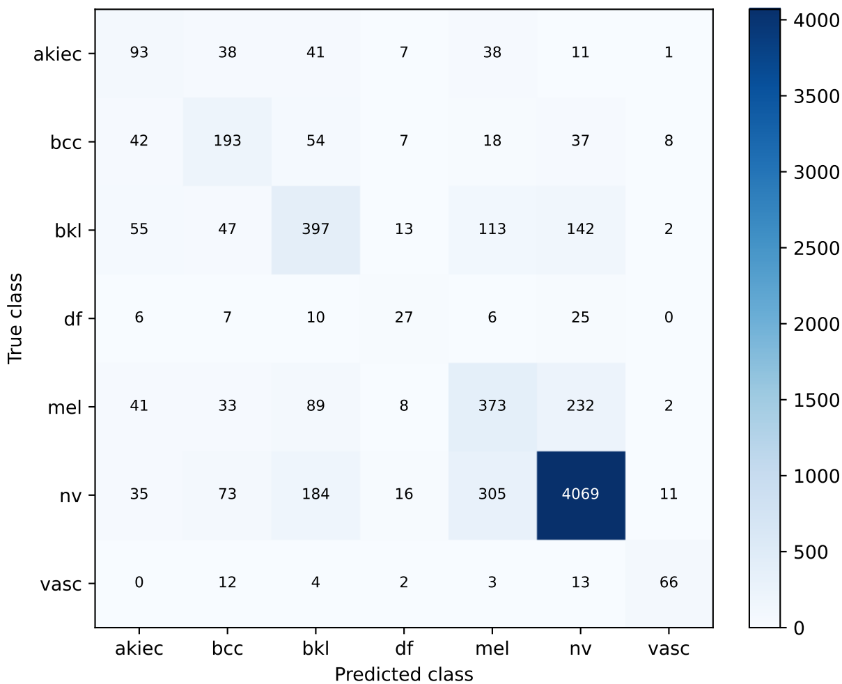
S67 ham_plus_external | train-only lesion-group OOF Confusion matrix
