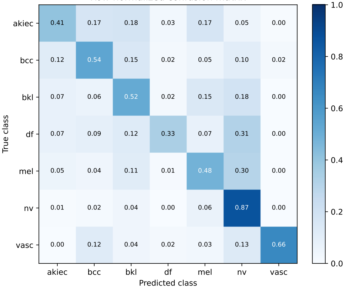
S67 ham_plus_external | train-only lesion-group OOF Row-normalized confusion matrix
