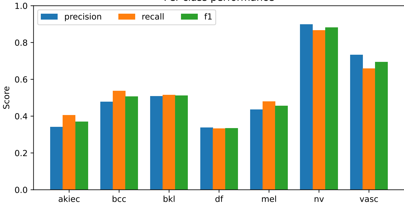
S67 ham_plus_external | train-only lesion-group OOF Per-class performance
