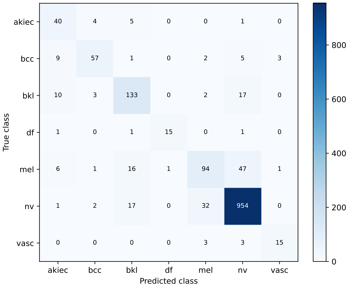
S39 ConvNeXt FP32 320px | strict development Confusion matrix
