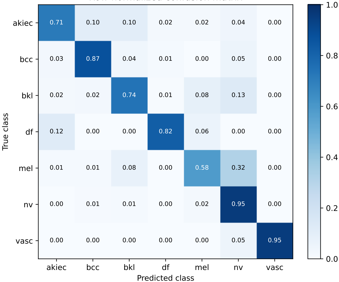
Frozen S83 equal-six | post-development test audit Row-normalized confusion matrix
