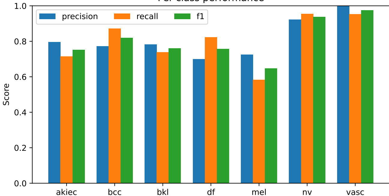
Frozen S83 equal-six | post-development test audit Per-class performance
