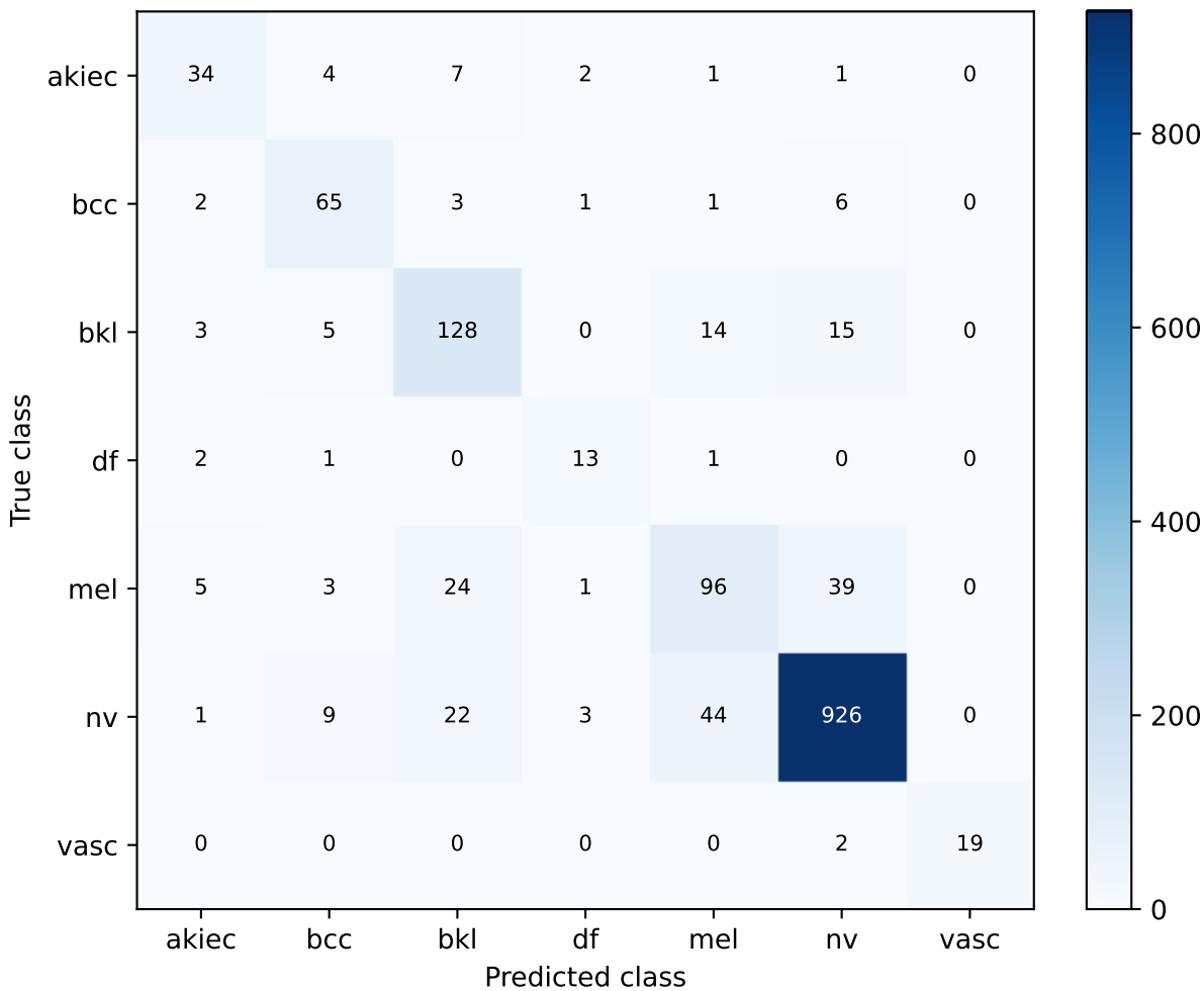
convnext_tiny | post-development test audit Confusion matrix
