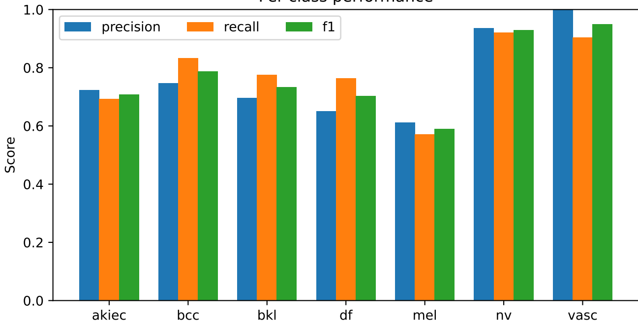
convnext_tiny | post-development test audit Per-class performance
