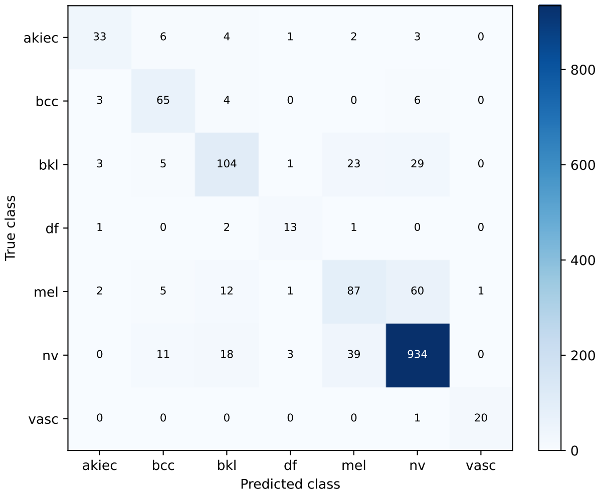
efficientnet_v2_s | post-development test audit Confusion matrix
