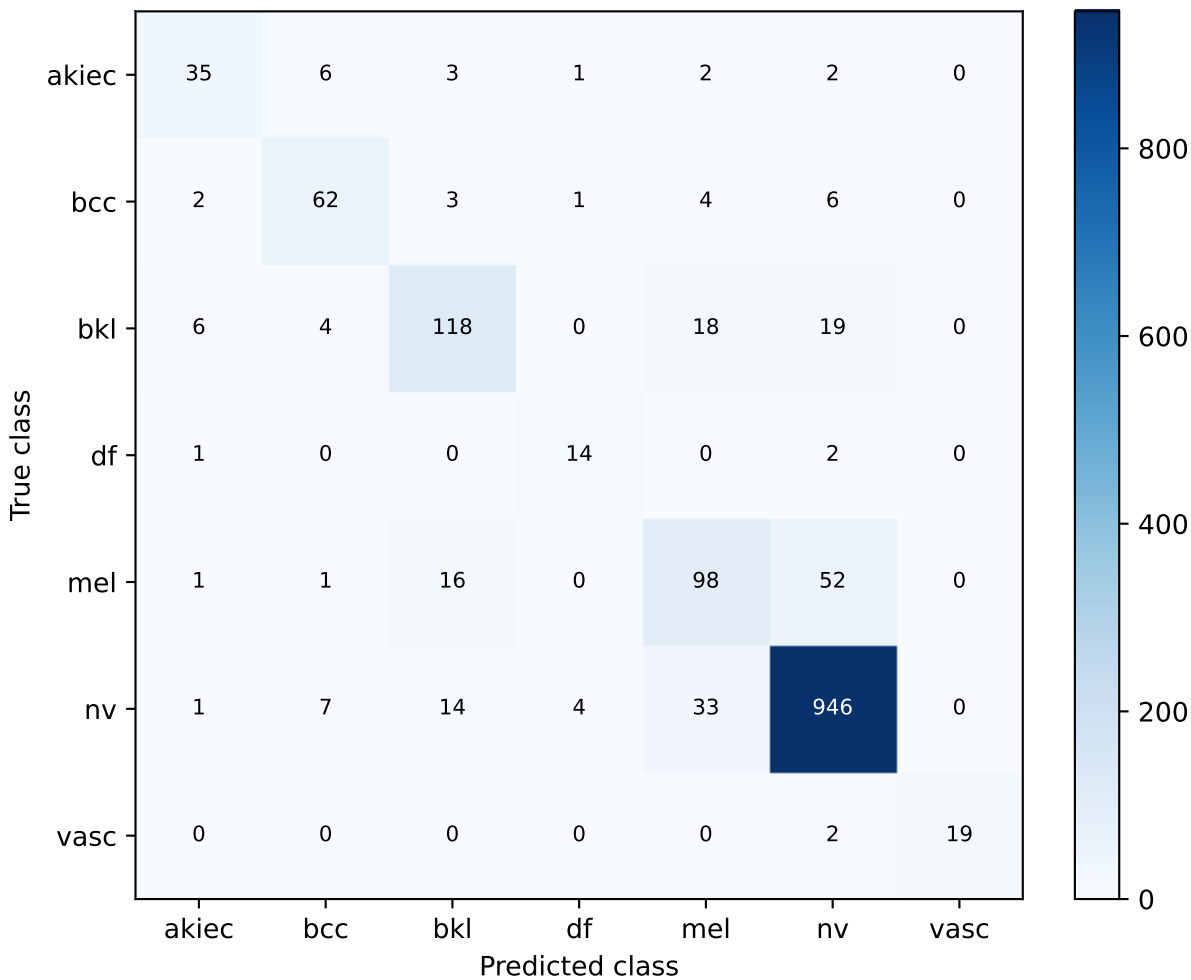
convnext_tiny + CBAM | post-development test audit Confusion matrix
