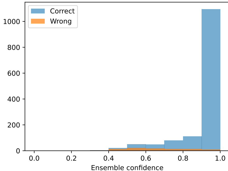
Confidence distributions
