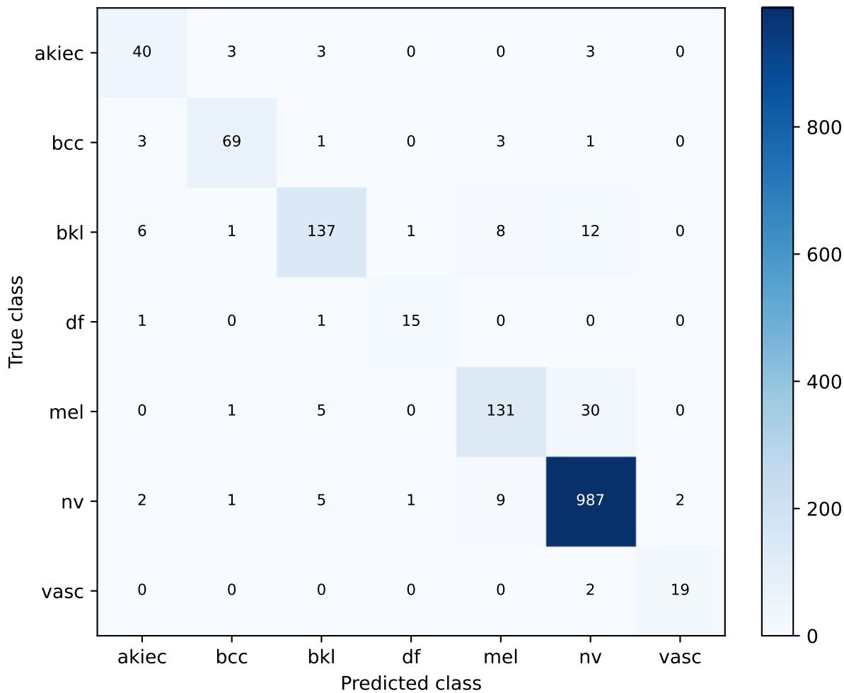
S79 exploratory validation Confusion matrix
