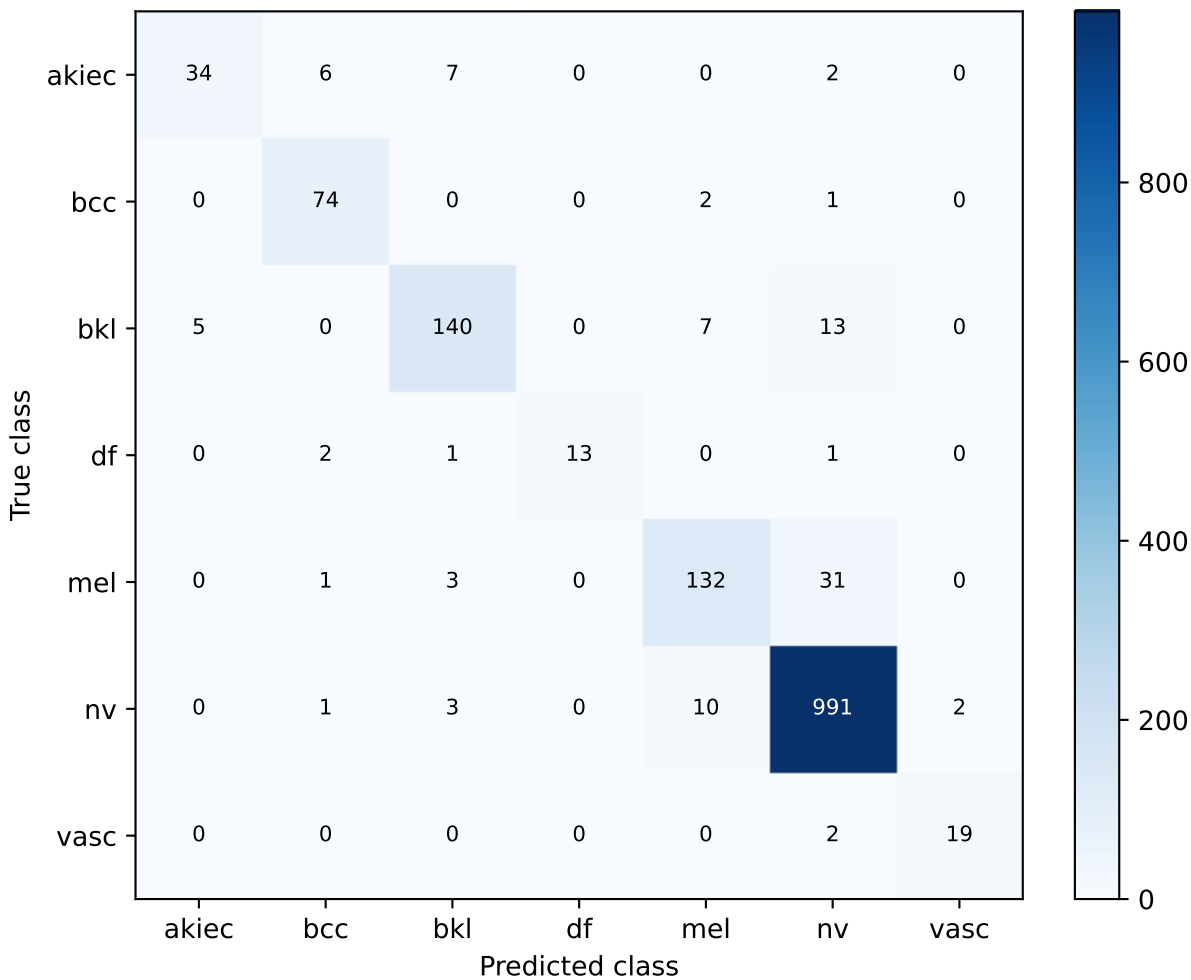
S79 replacement equal-five | exploratory validation Confusion matrix
