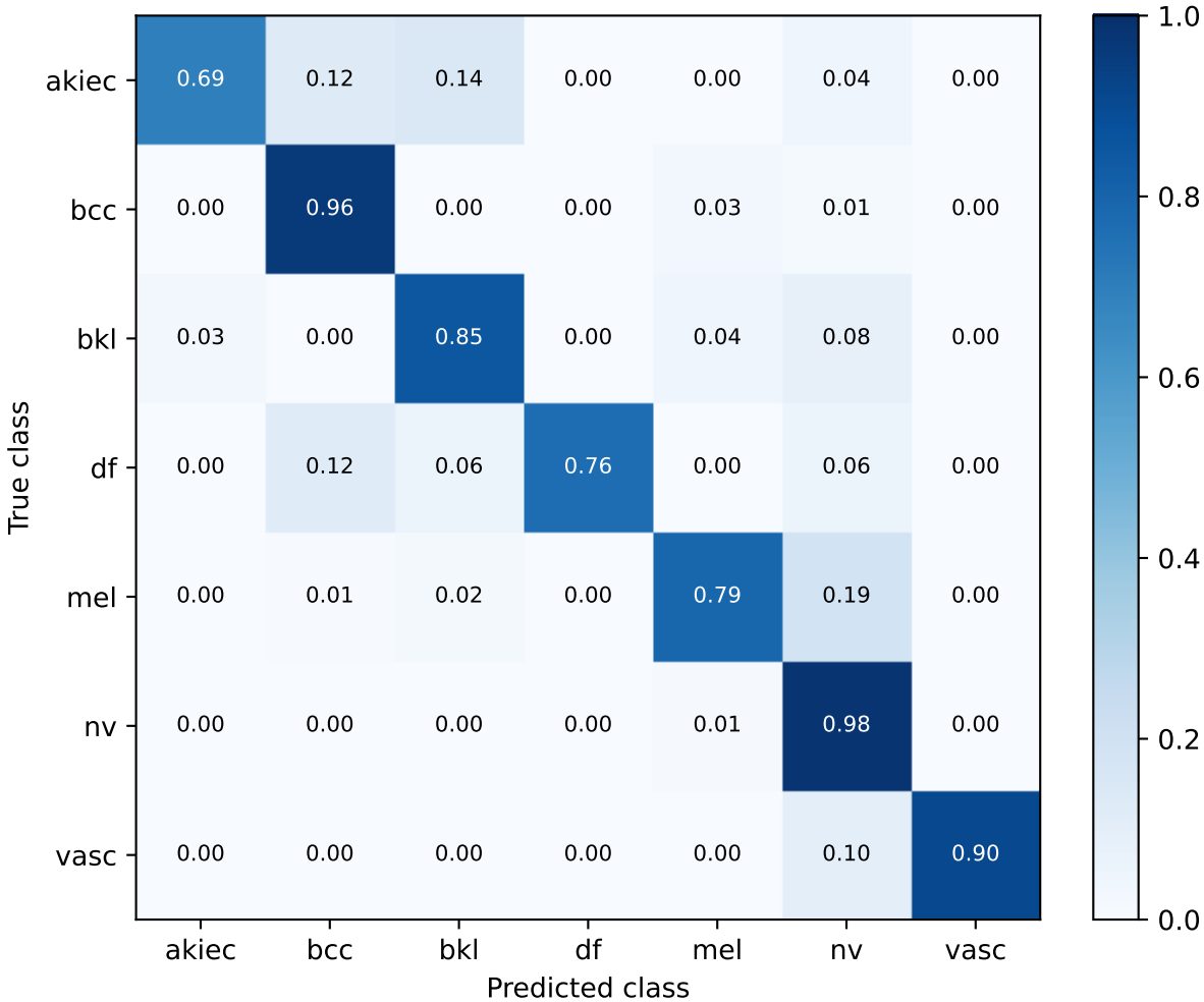
S79 replacement equal-five | exploratory validation Row-normalized confusion matrix
