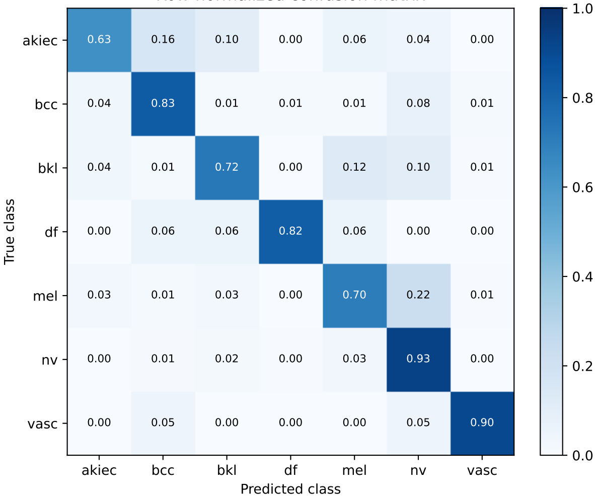
efficientnet_b0 | exploratory_image_level validation Row-normalized confusion matrix
