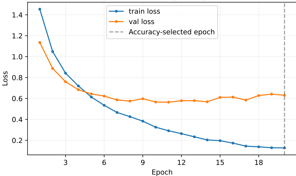
efficientnet_b0 | exploratory_image_level validation
