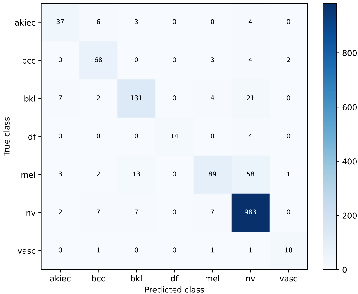
S40 fixed equal ensemble; strict development Confusion matrix
