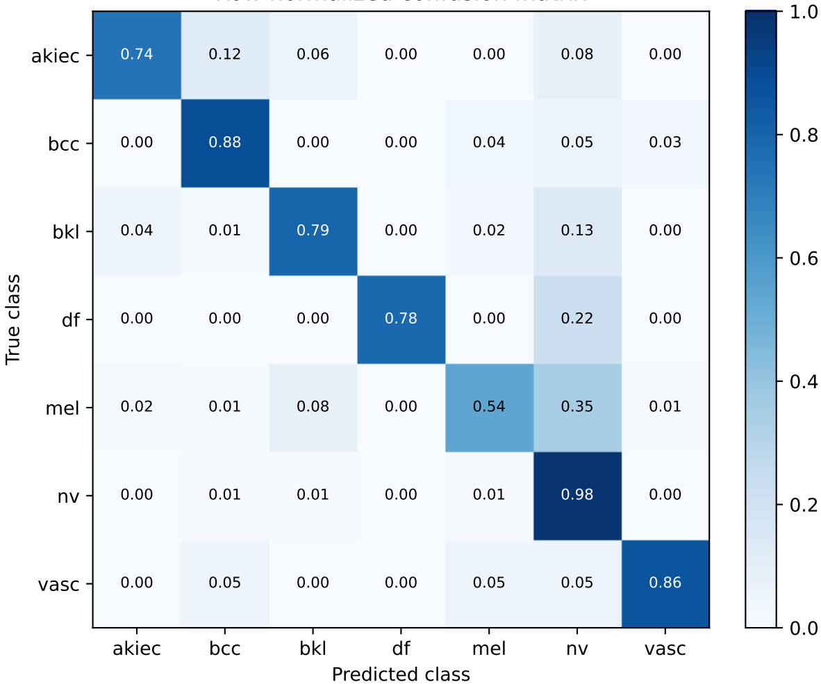
S40 fixed equal ensemble; strict development Row-normalized confusion matrix
