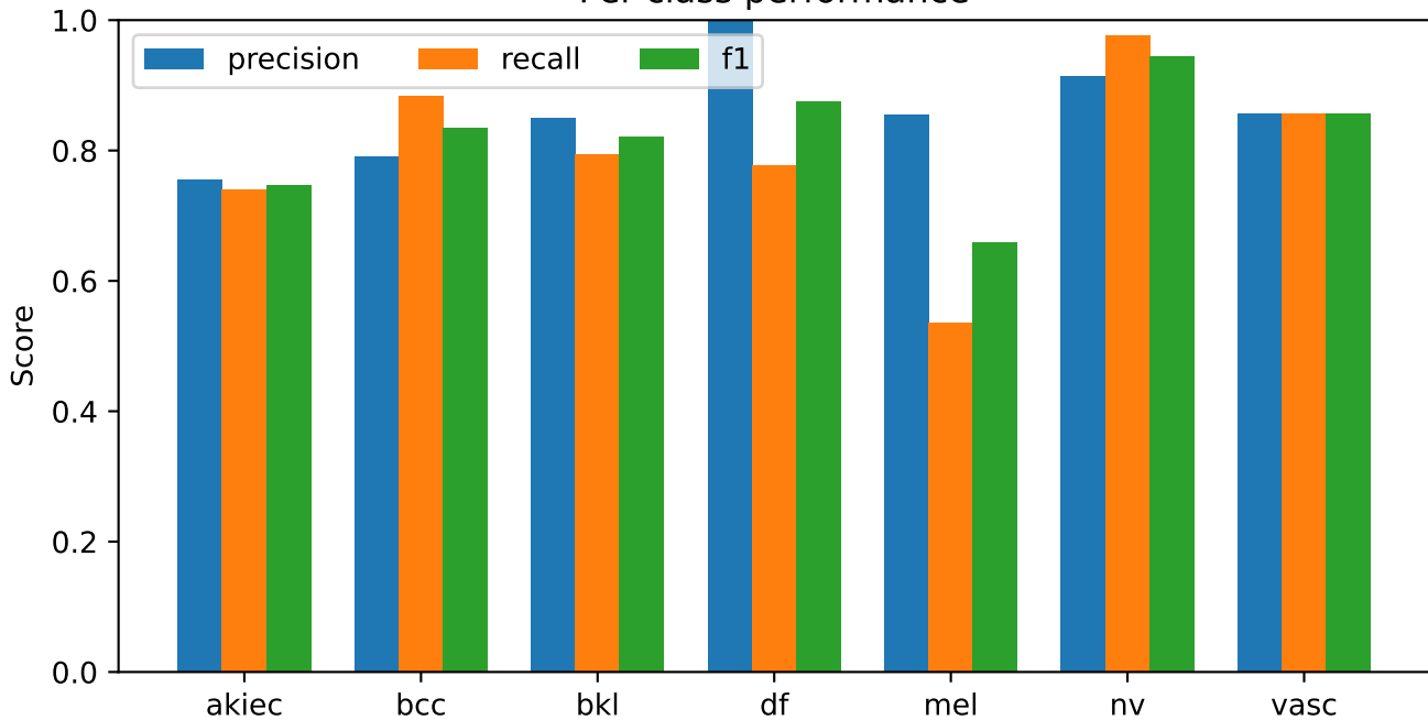
S40 fixed equal ensemble; strict development Per-class performance
