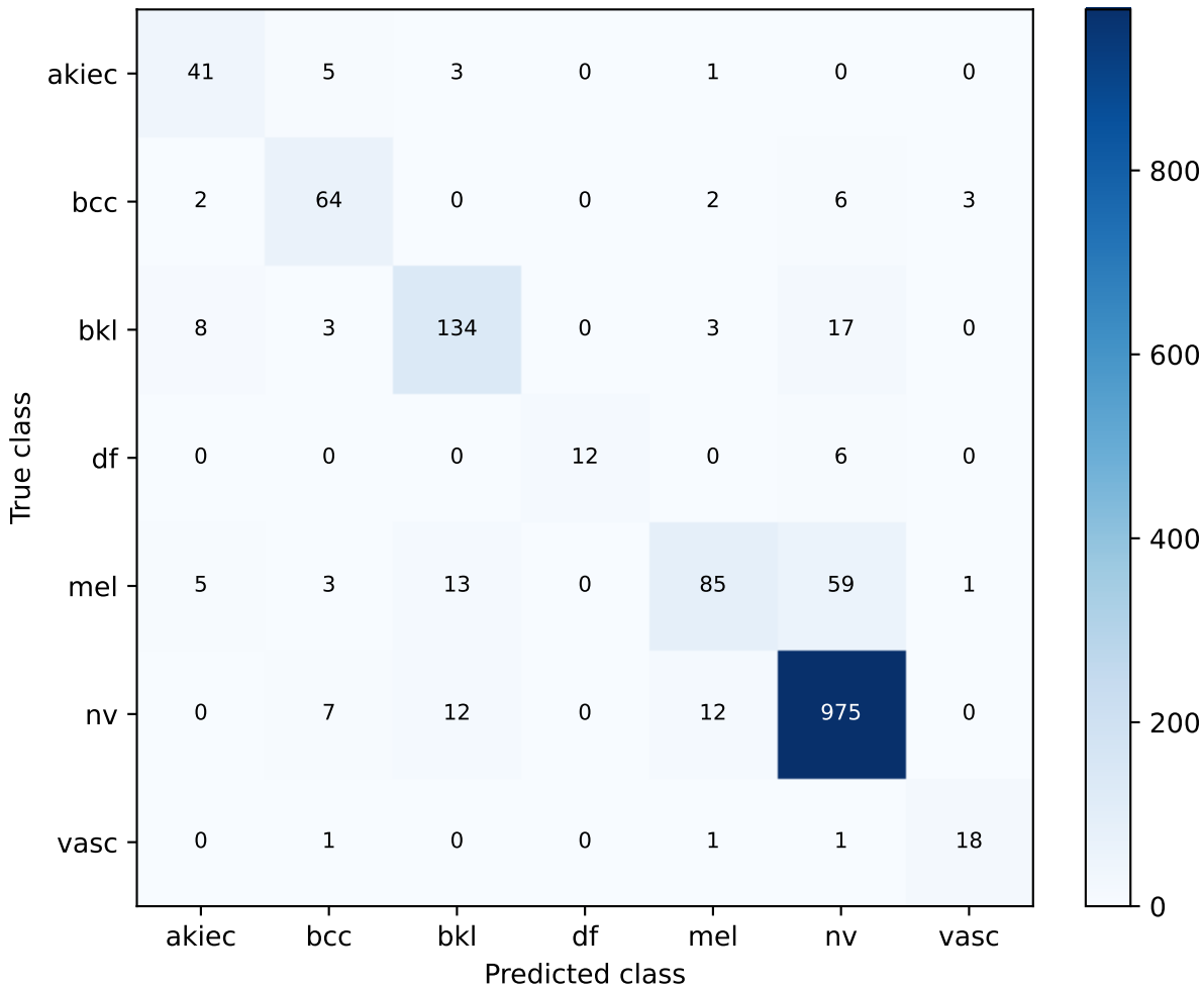
S40 Mixup | strict development Confusion matrix
