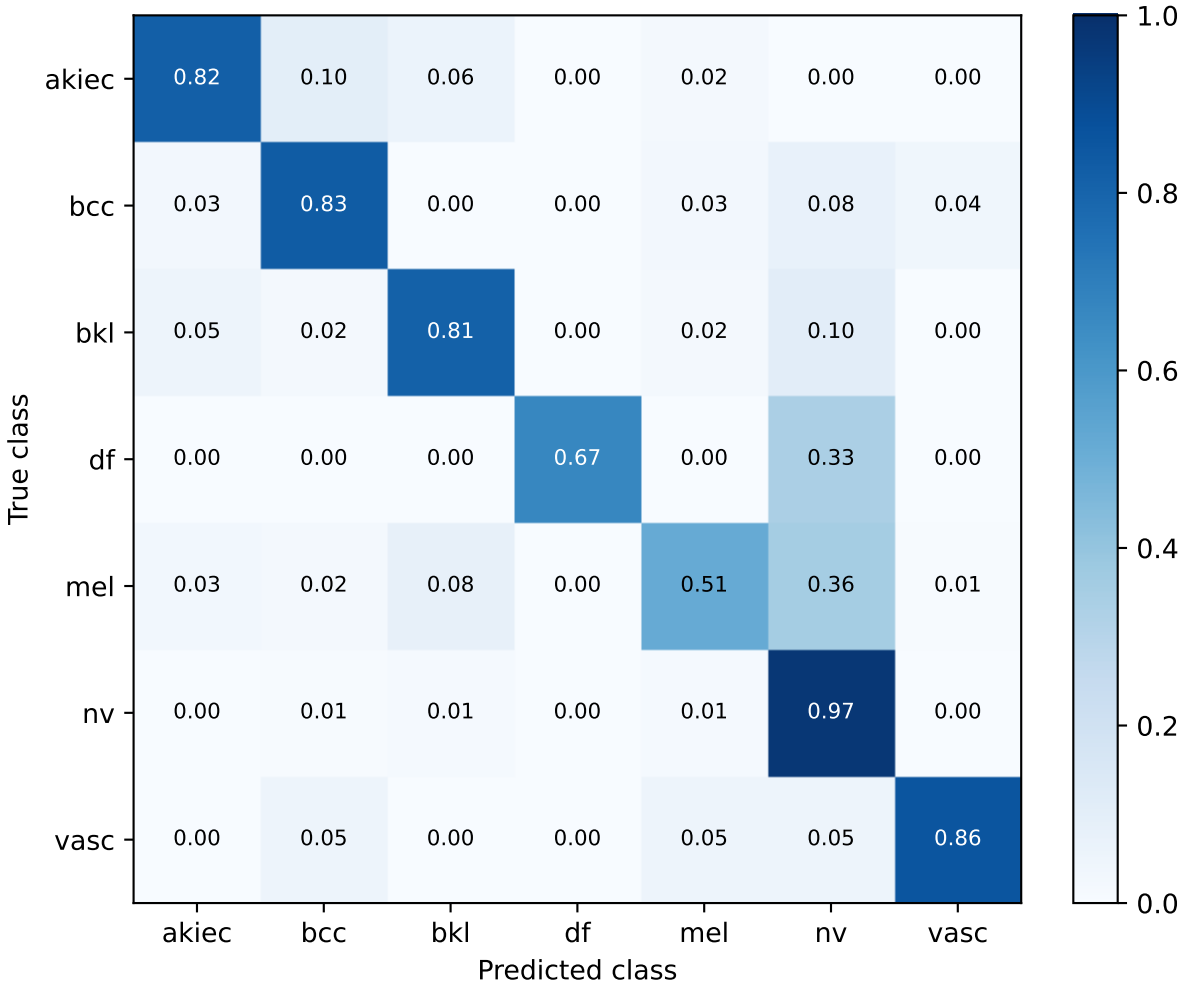
S40 Mixup | strict development Row-normalized confusion matrix
