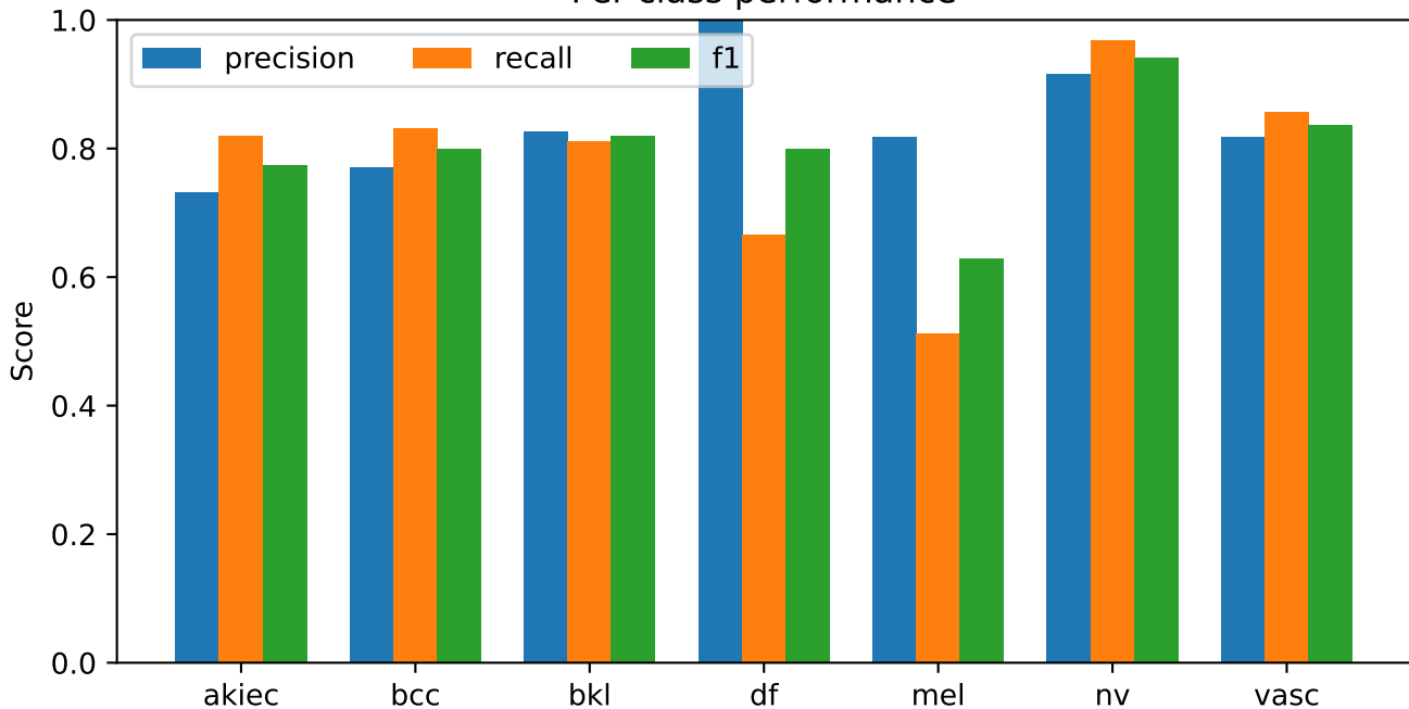
S40 Mixup | strict development Per-class performance
