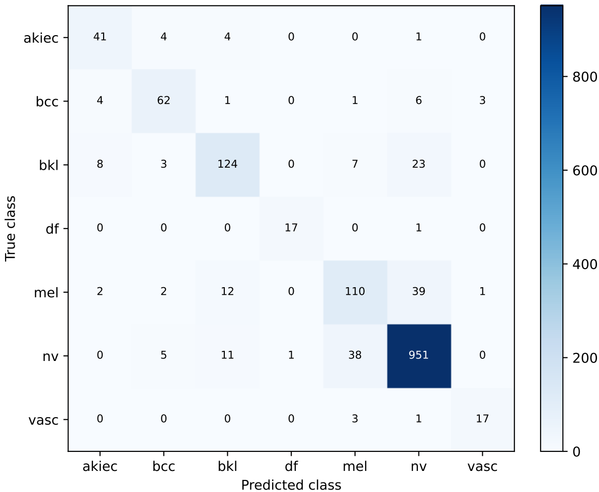
S40 Mixup | strict development_macro_f1 Confusion matrix
