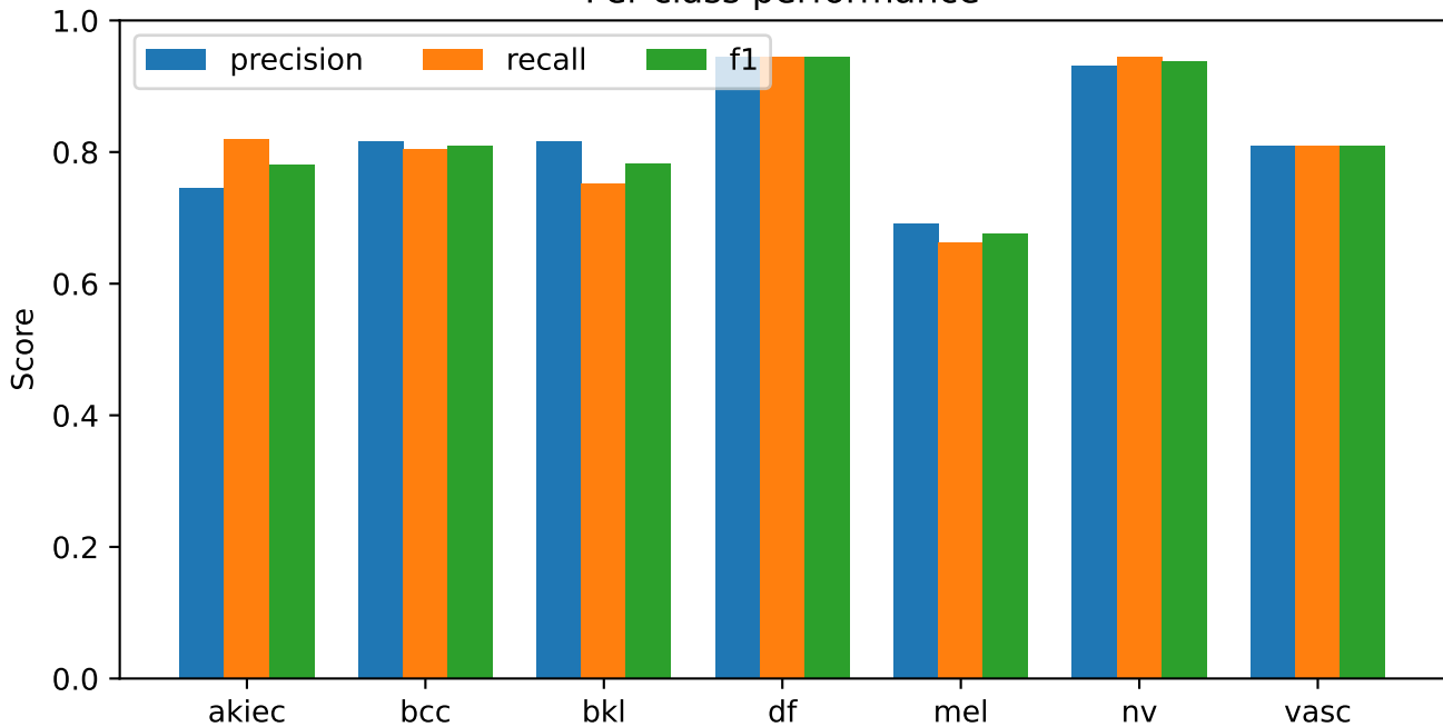
S40 Mixup | strict development_macro_f1 Per-class performance
