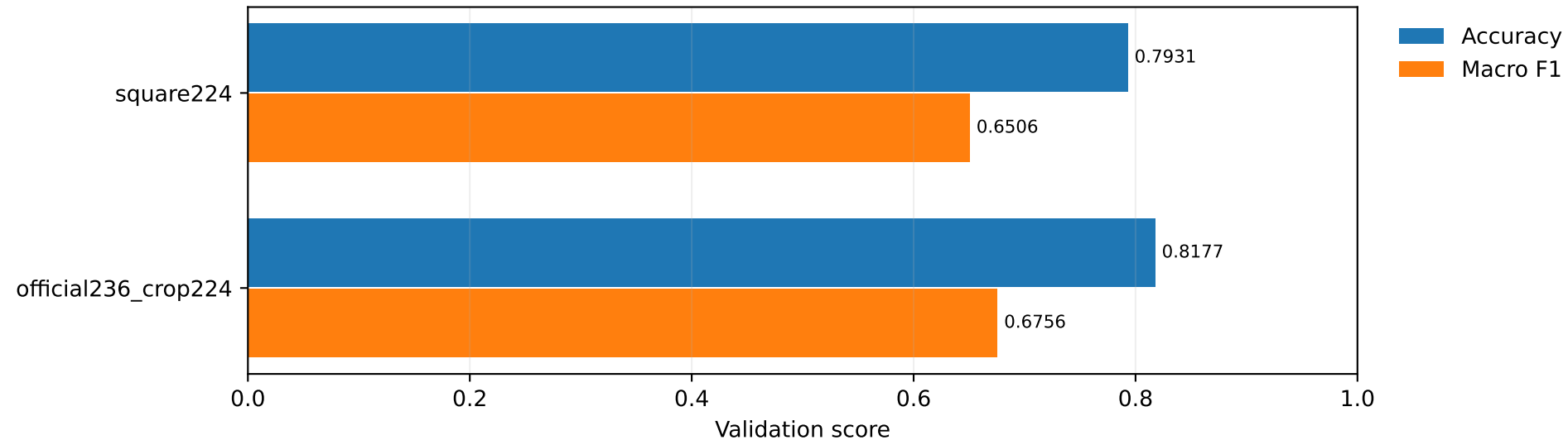
S64 paired CPU pretrained-feature preprocessing screen
