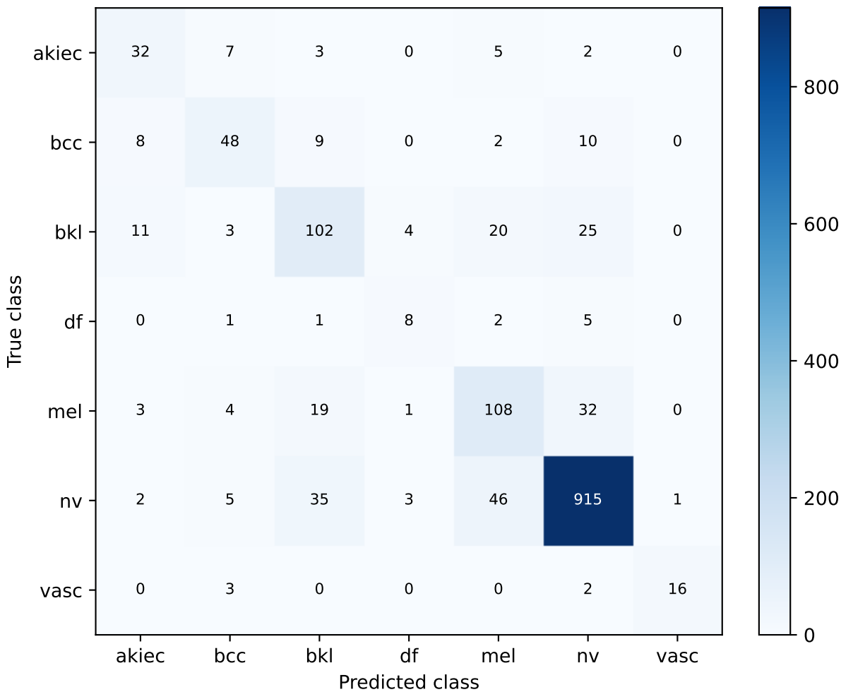
S64 official236_crop224: frozen features, exploratory validation Confusion matrix
