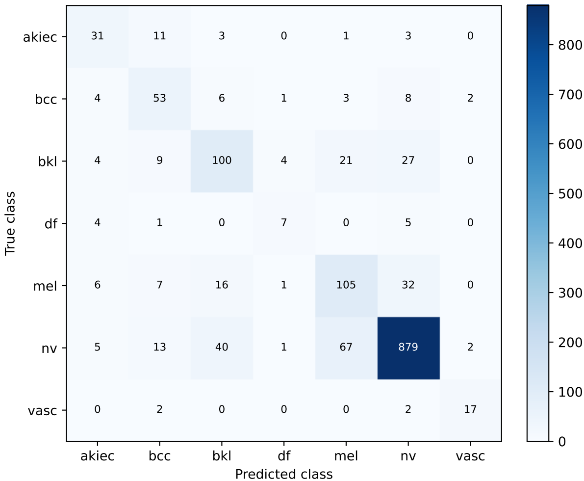
S64 square224: frozen features, exploratory validation Confusion matrix
