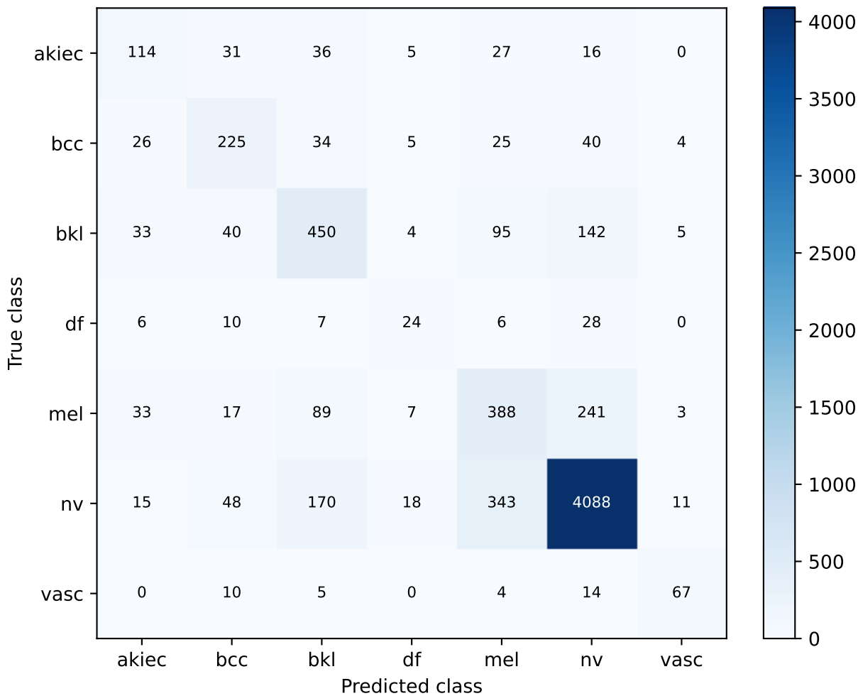
S65 official236_crop224 | train-only lesion-group OOF Confusion matrix
