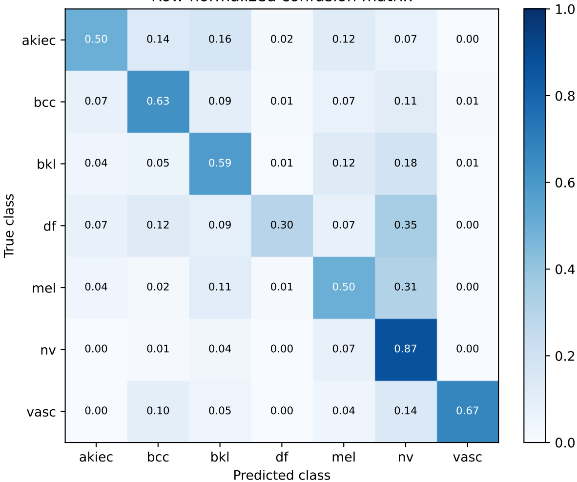
S65 official236_crop224 | train-only lesion-group OOF Row-normalized confusion matrix
