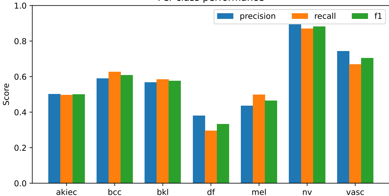
S65 official236_crop224 | train-only lesion-group OOF Per-class performance
