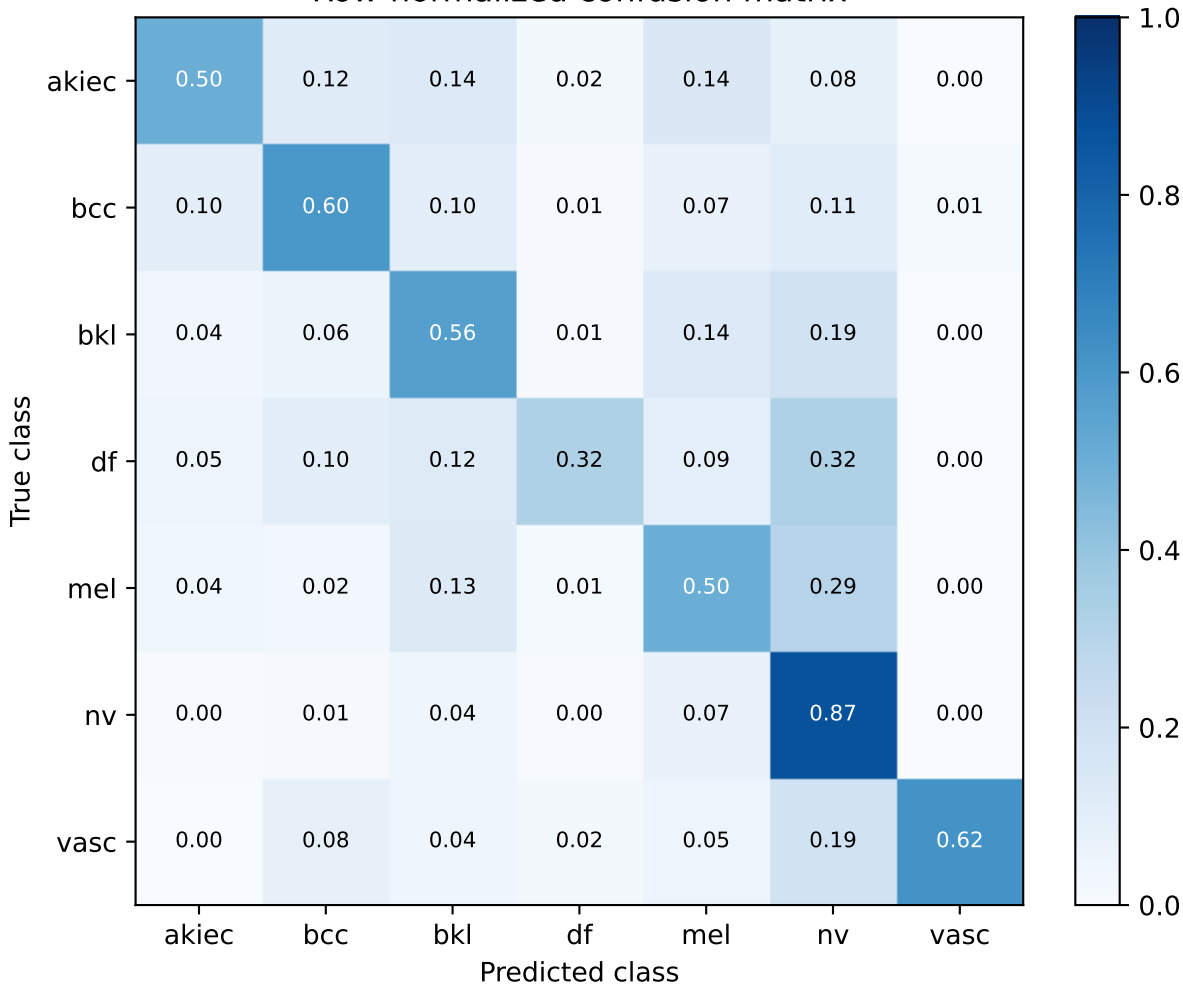
S65 square224 | train-only lesion-group OOF Row-normalized confusion matrix
