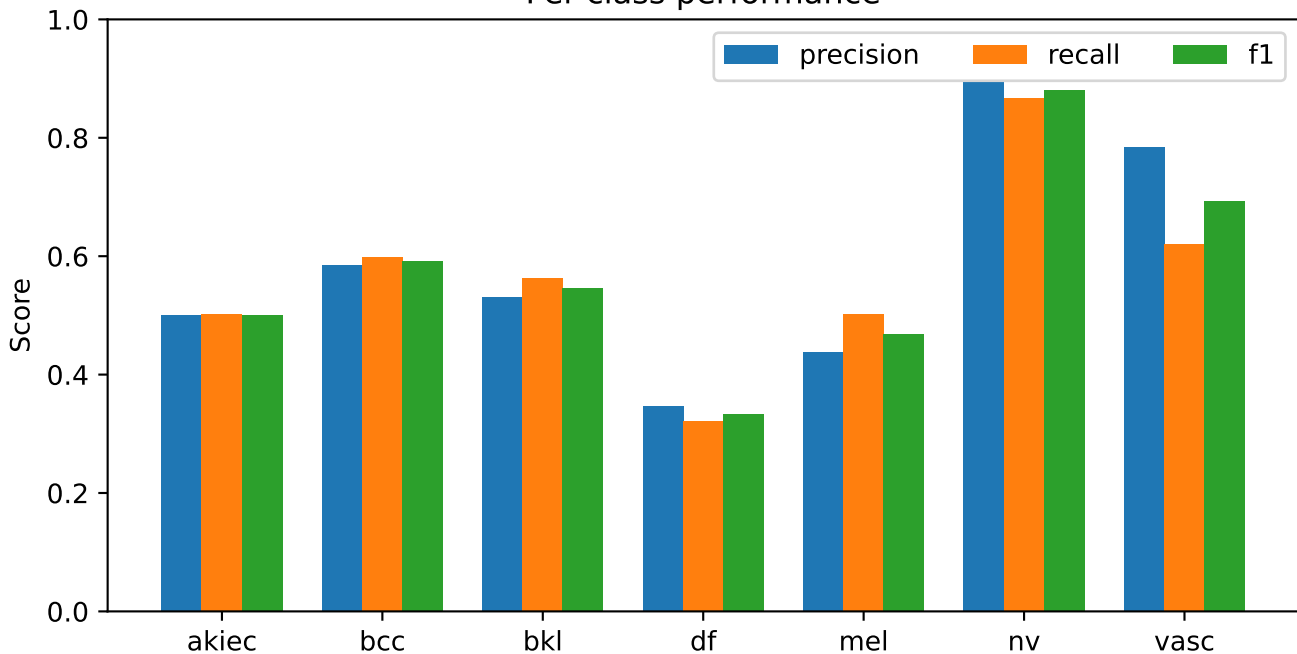
S65 square224 | train-only lesion-group OOF Per-class performance
