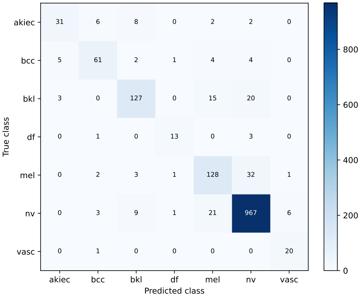
densenet201 | exploratory_image_level validation Confusion matrix
