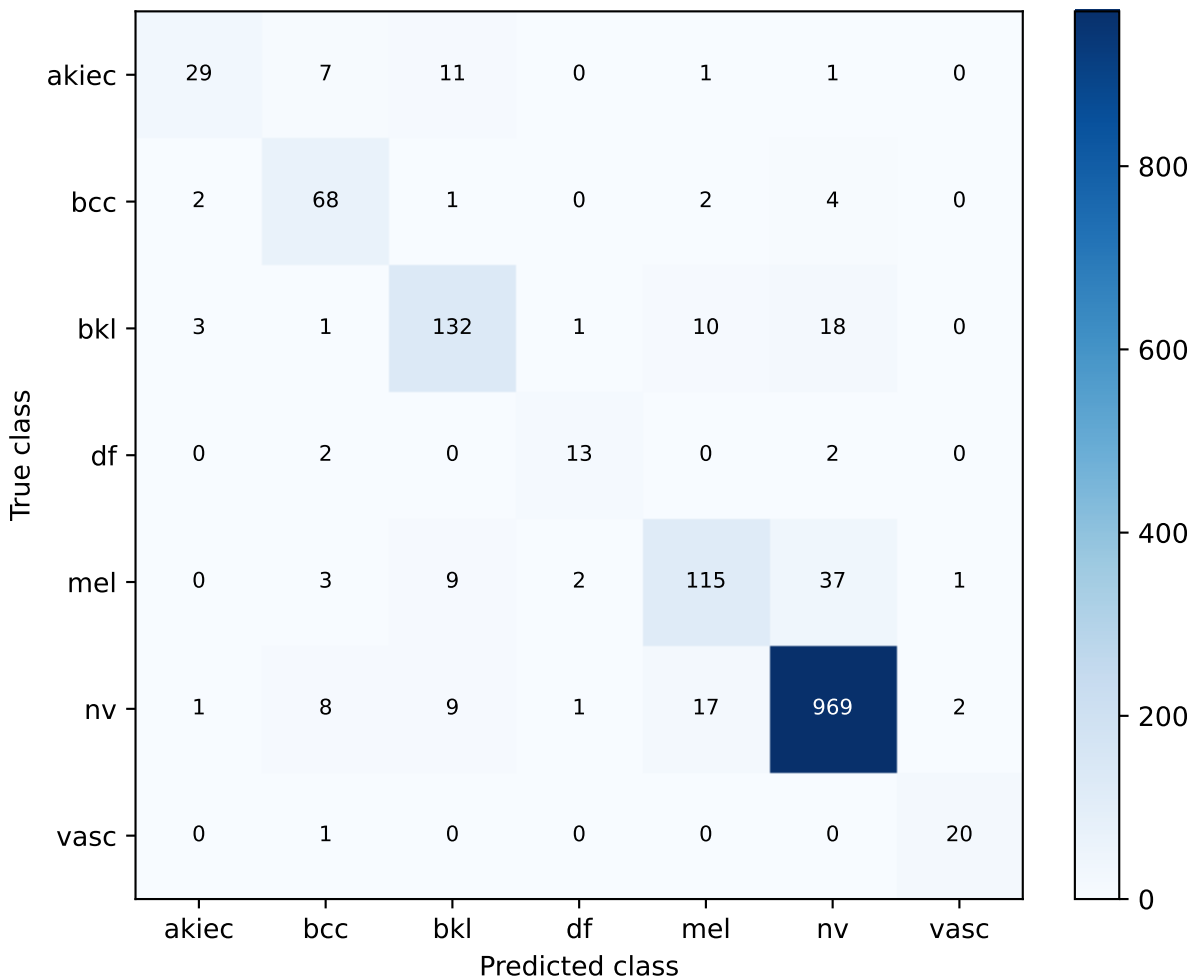
S15 DenseNet201 | exploratory validation | macro-F1 winner Confusion matrix
