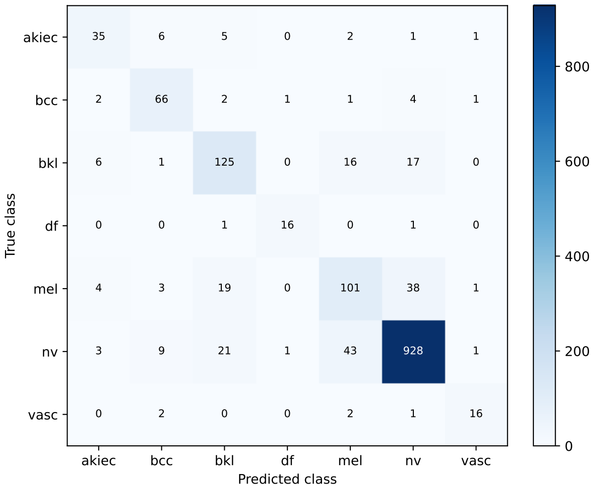
efficientnet_b0 | strict_lesion_disjoint validation Confusion matrix
