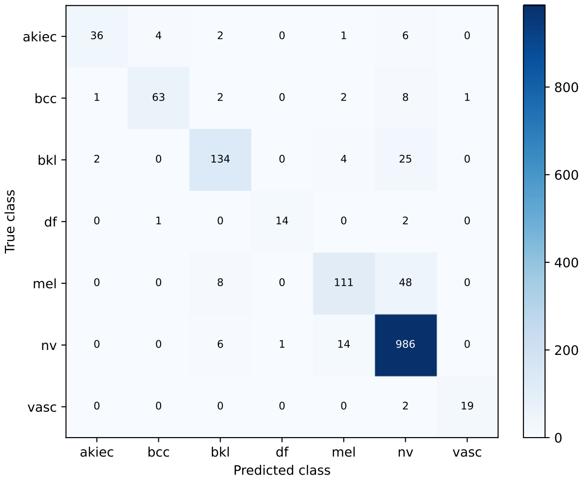
S89 Swin-Tiny | exploratory validation Confusion matrix
