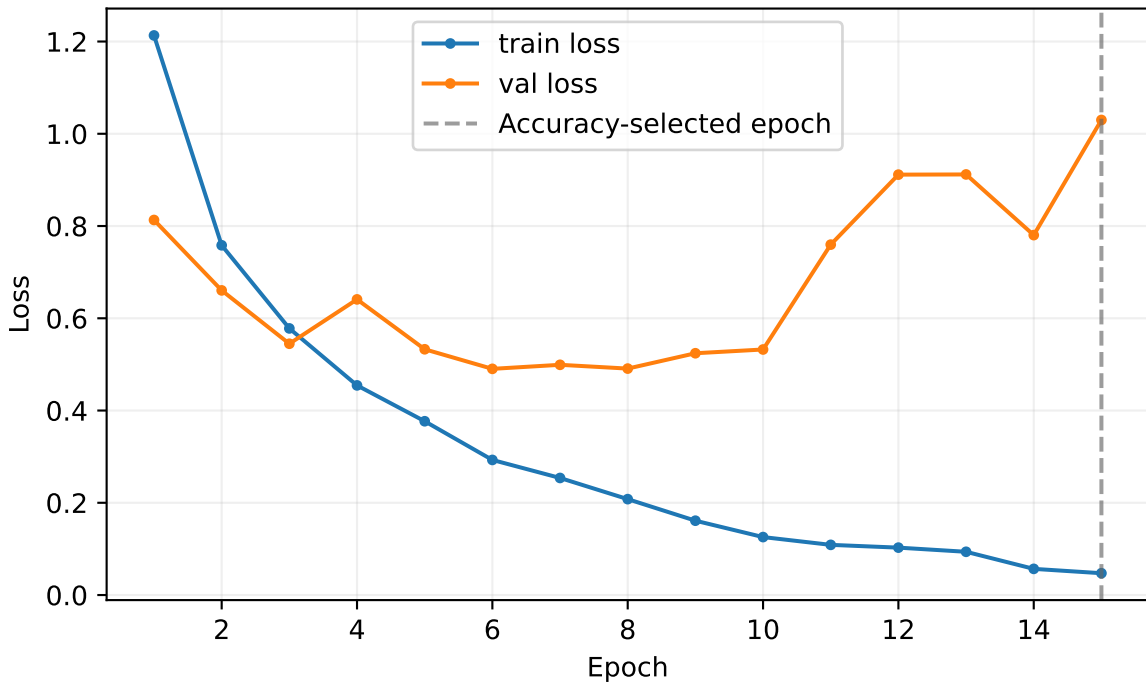
S89 Swin-Tiny training
