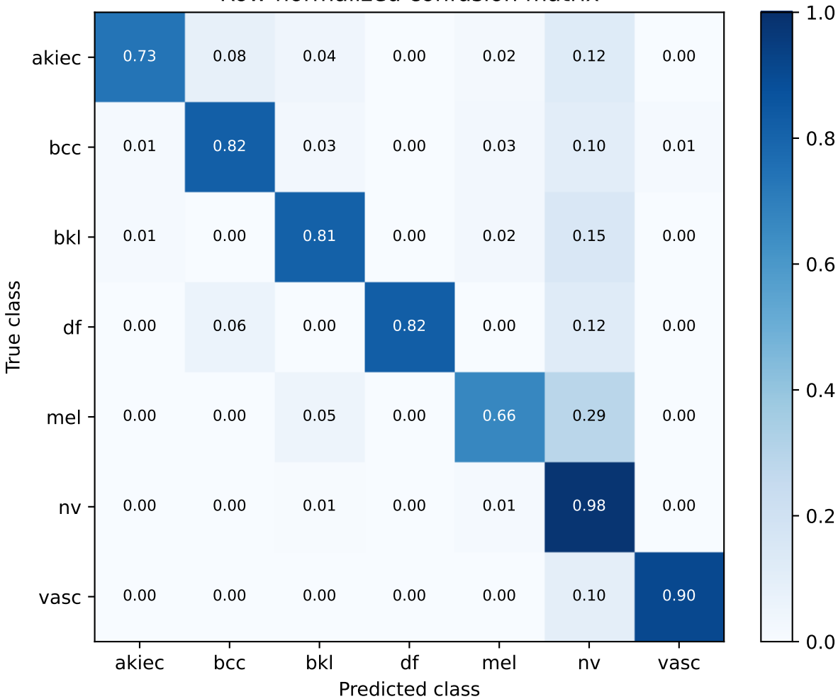
S89 Swin-Tiny final committed epoch | exploratory validation Row-normalized confusion matrix
