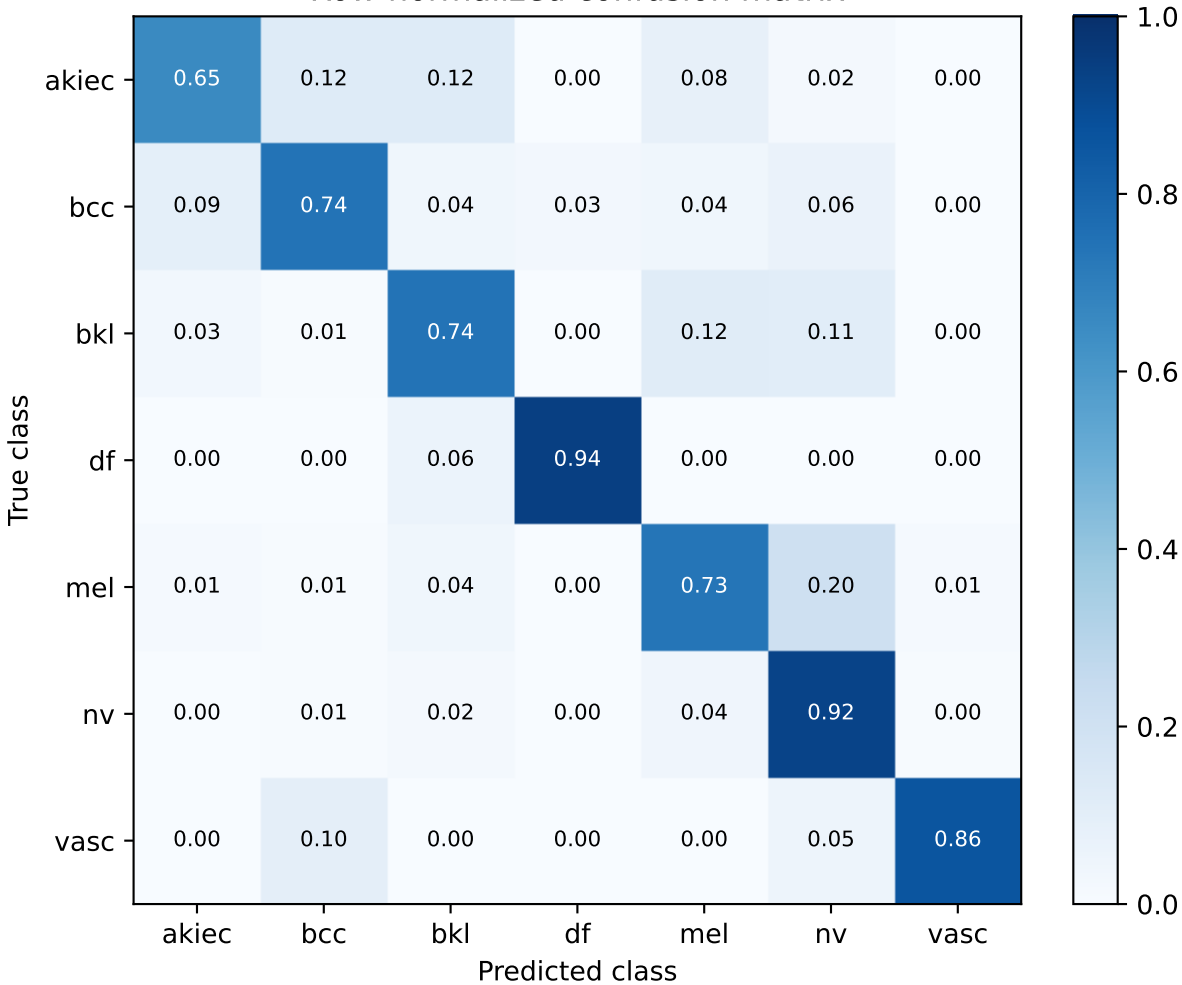
S05 B0+CBAM | exploratory validation | macro-F1 winner Row-normalized confusion matrix
