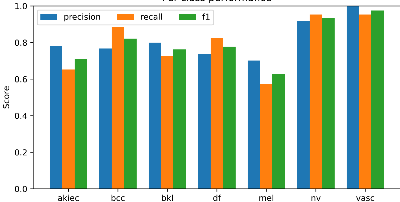
Fixed S80 equal-five | post-development test audit Per-class performance
