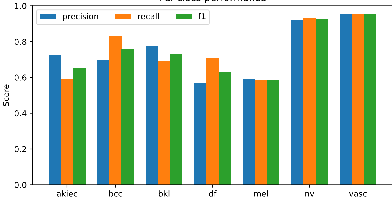
convnext_small | post-development test audit Per-class performance
