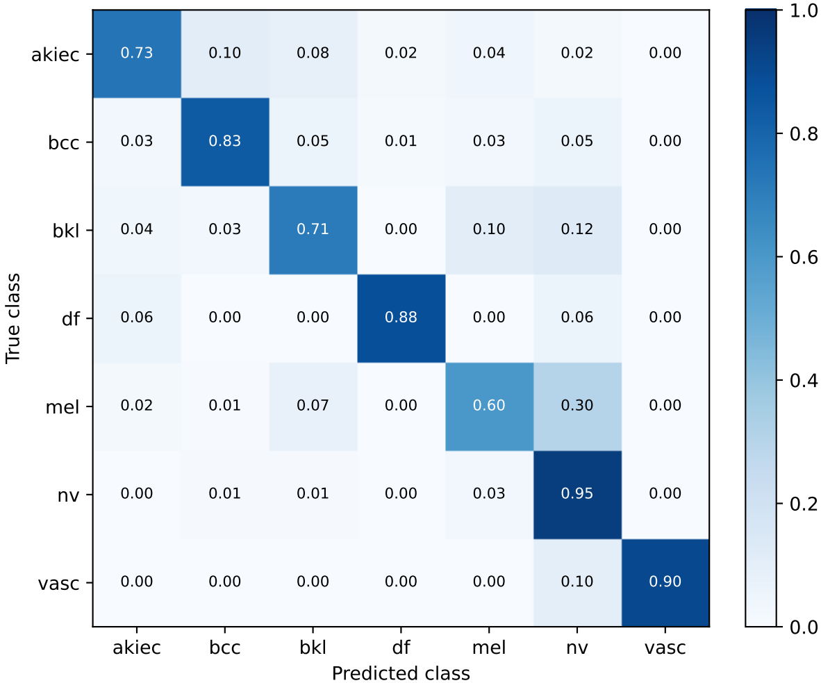
convnext_tiny + CBAM | post-development test audit Row-normalized confusion matrix
