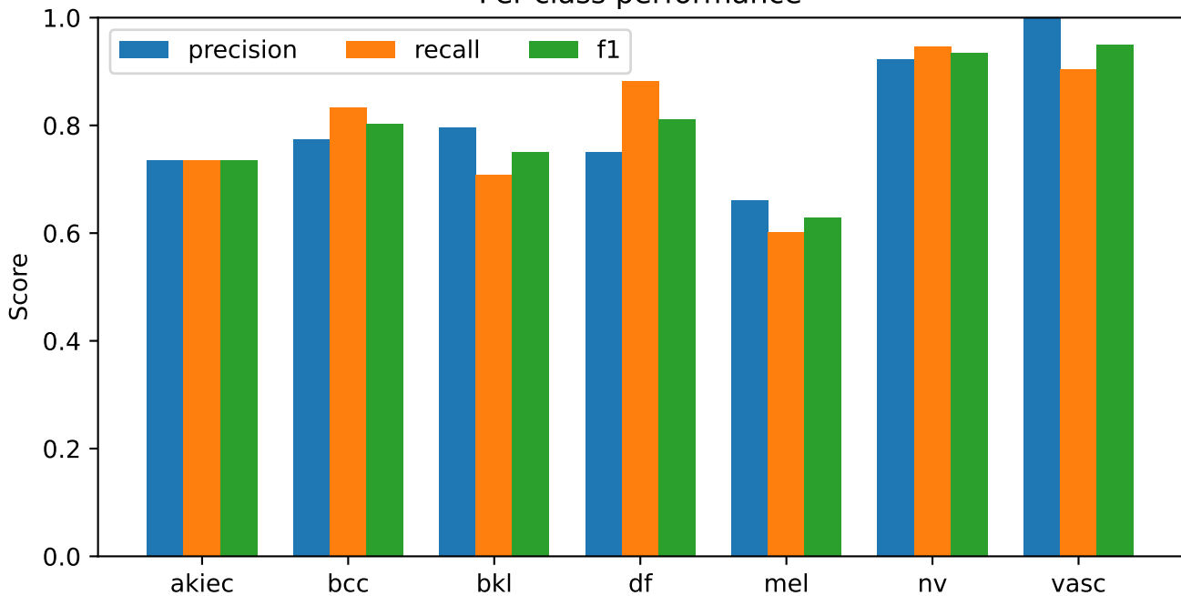
convnext_tiny + CBAM | post-development test audit Per-class performance
