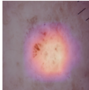
efficientnet_v2_s
