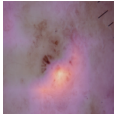
convnext_small
