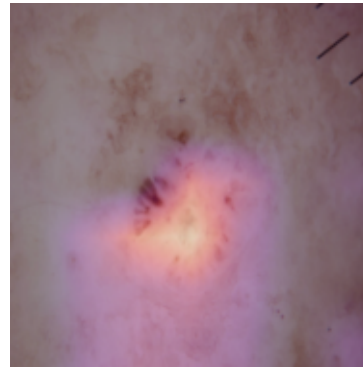
convnext_tiny + CBAM
