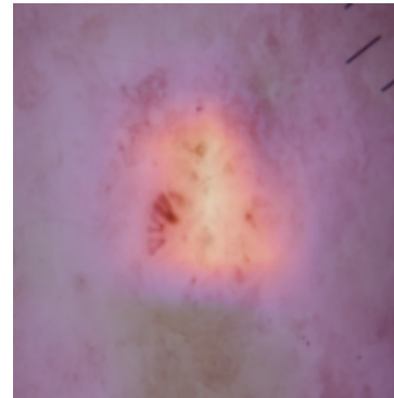
efficientnet_b0
