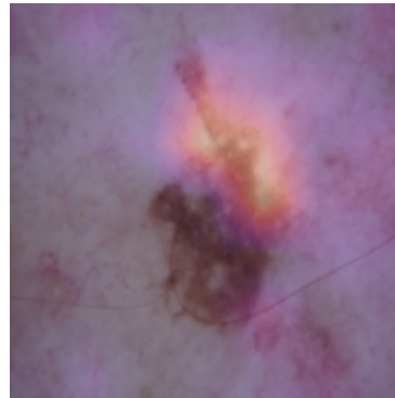
convnext_small
