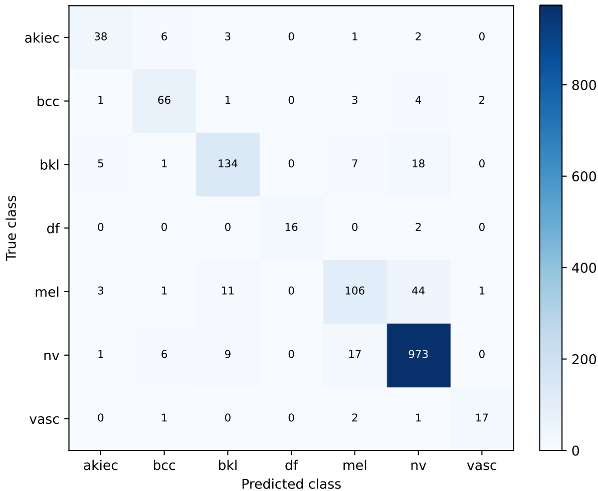
crossfit_regularized_class_bias | post-test development CPU screening Confusion matrix
